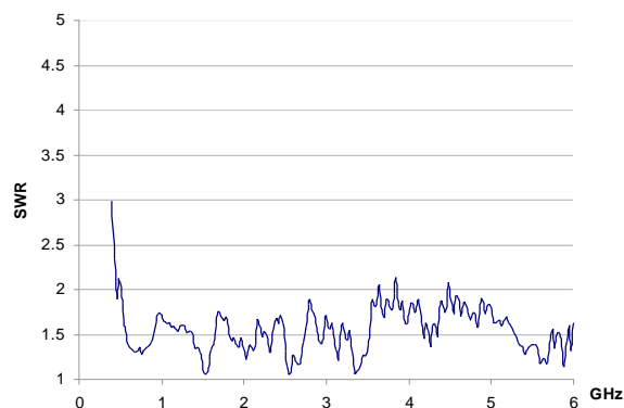
UAVee™ 6000 has excellent SWR over a very wide frequency range
